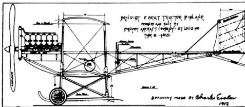
Eisler's original drawing in 1912 for the plane later built by Benoist students that year.
